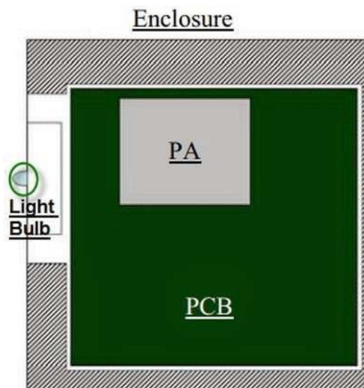
Fig.1. Construction of LiFi assembly [3]
